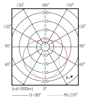
Light Distribution Diagram - MAS LEDtube HF 1200mm HE 16.5W 865 T5
