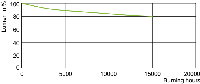
Lumen Maintenance Diagram - MC CDM-R Elite 70W/930 E27 PAR30L 10D
