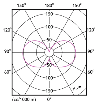
Light Distribution Diagram - MAS LEDBulbND5.2-75W E27 830 A60 FR G UE
