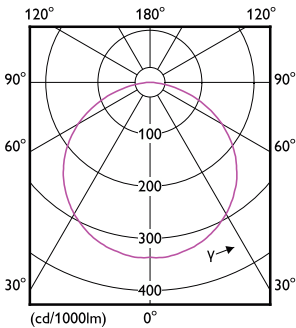
Light Distribution Diagram - MAS LEDstrip 12.5W940 1500LM/M 5M
