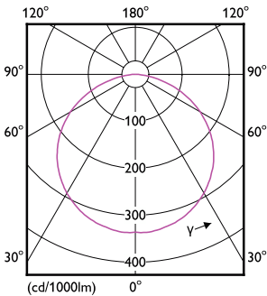
Light Distribution Diagram - MAS LEDstrip 12.5W965 1450LM/M 5M
