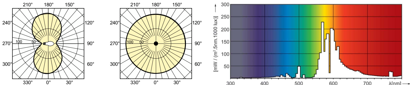
Light Distribution Diagram - MST SON APIA Plus Xtra 100W E40 1SL/12
