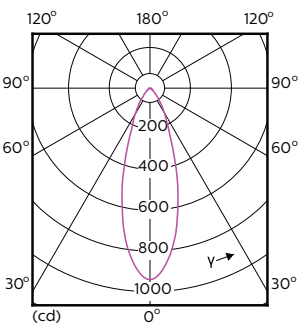
Light Distribution Diagram - MAS LED ExpertColor 5.5-50W GU10 940 36D
