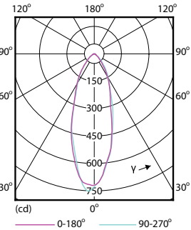
Light Distribution Diagram - Corepro LEDspot 4.6-50W GU10 865 36D
