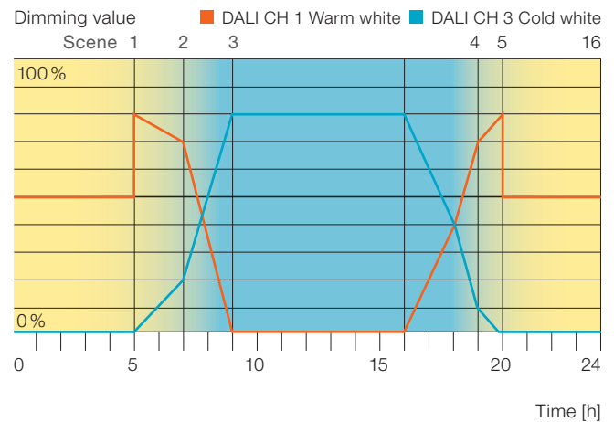
Automatic operation: Dimming behavior of the Tunable White luminaires according to the time of day
