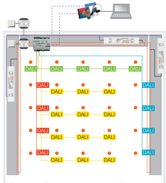
Salesroom with control components
